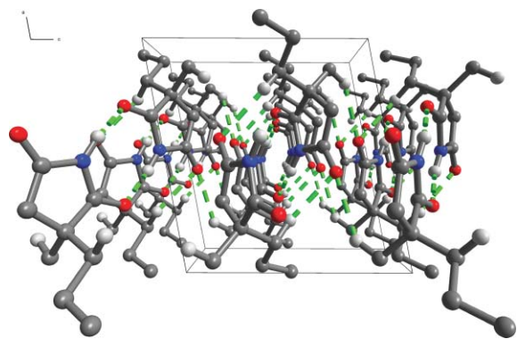
Fig. 6 Crystal structure of (II). Only H atoms involved in hydrogen bonding (indicated by dashed lines) are shown. Selected intermolecular distances: N(H)⋯O, 2.80(1) Å; C(H)⋯O, 3.49(1) and 3.49(1) Å.
